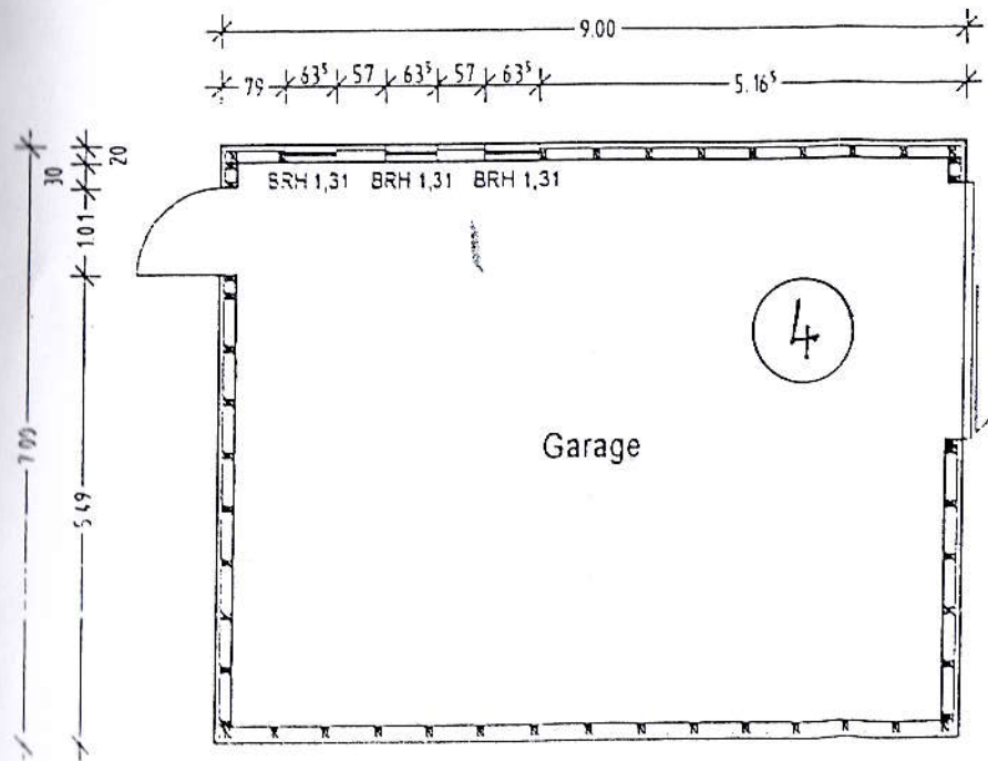
GRUNDRISS GARAGE
